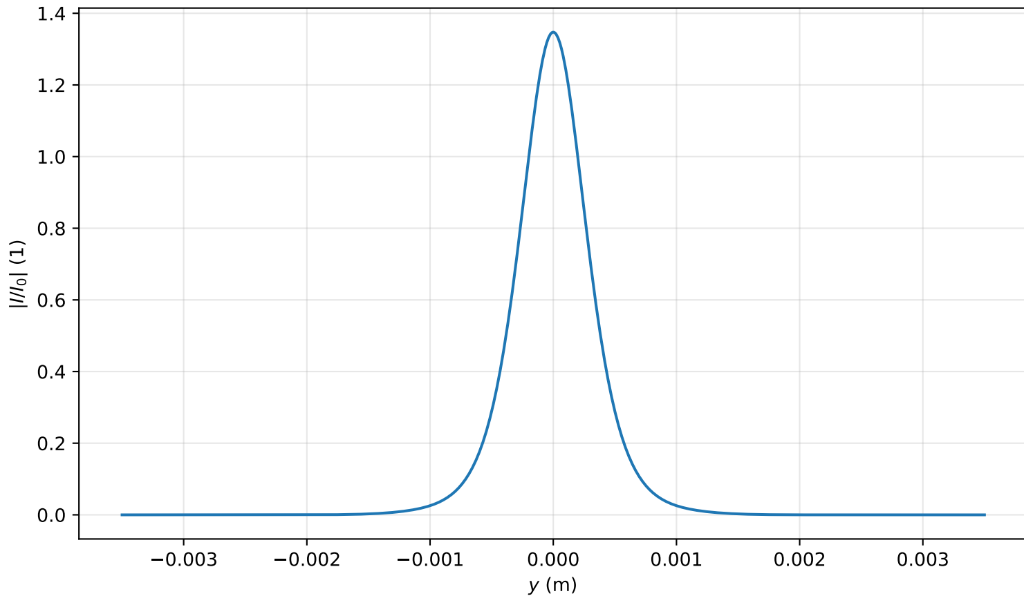
Intensity profile I(x=0, y, z=1.751)/I_0 , P_{in}=0.8P_{cr} , artificial time
